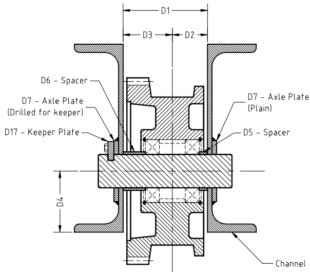
Double Flange Wheel Assembly - Imperial Dimensions
