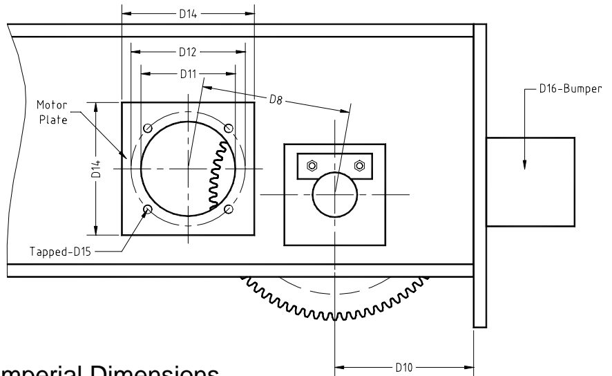
Double Flange Wheel Assembly - Imperial Dimensions
