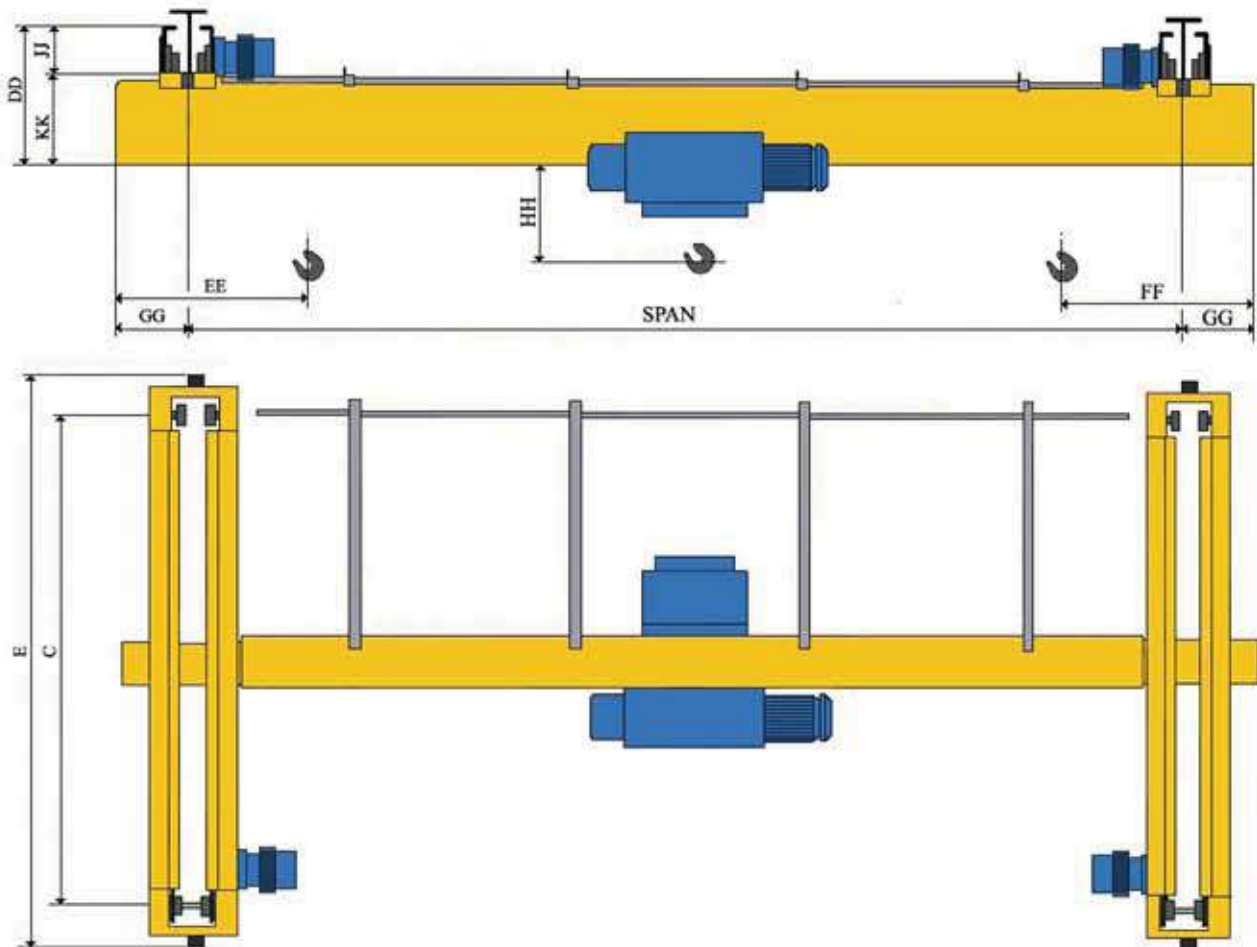
Motorized Single Girder Underslung Crane Bridge TYPE UR-S
